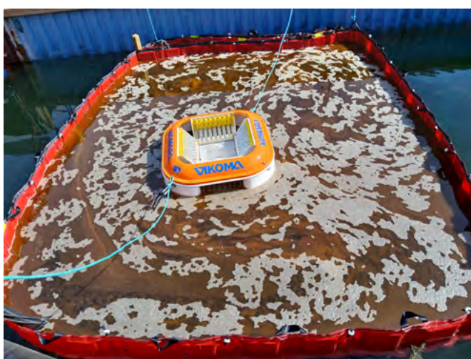
Figure 8. Komara Midi 4 disc skimmer in calm waters at the beginning and end of a skimming operation. The skimmer removed virtually all of the diesel oil without having to change position or assist with the oil supply. Photos: Justiina Halonen, 2025.
